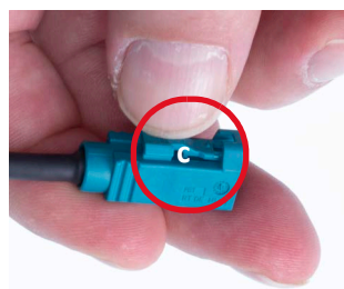
Figure 6: Pressing down the latch (c) of the FAKRA coaxial connector
