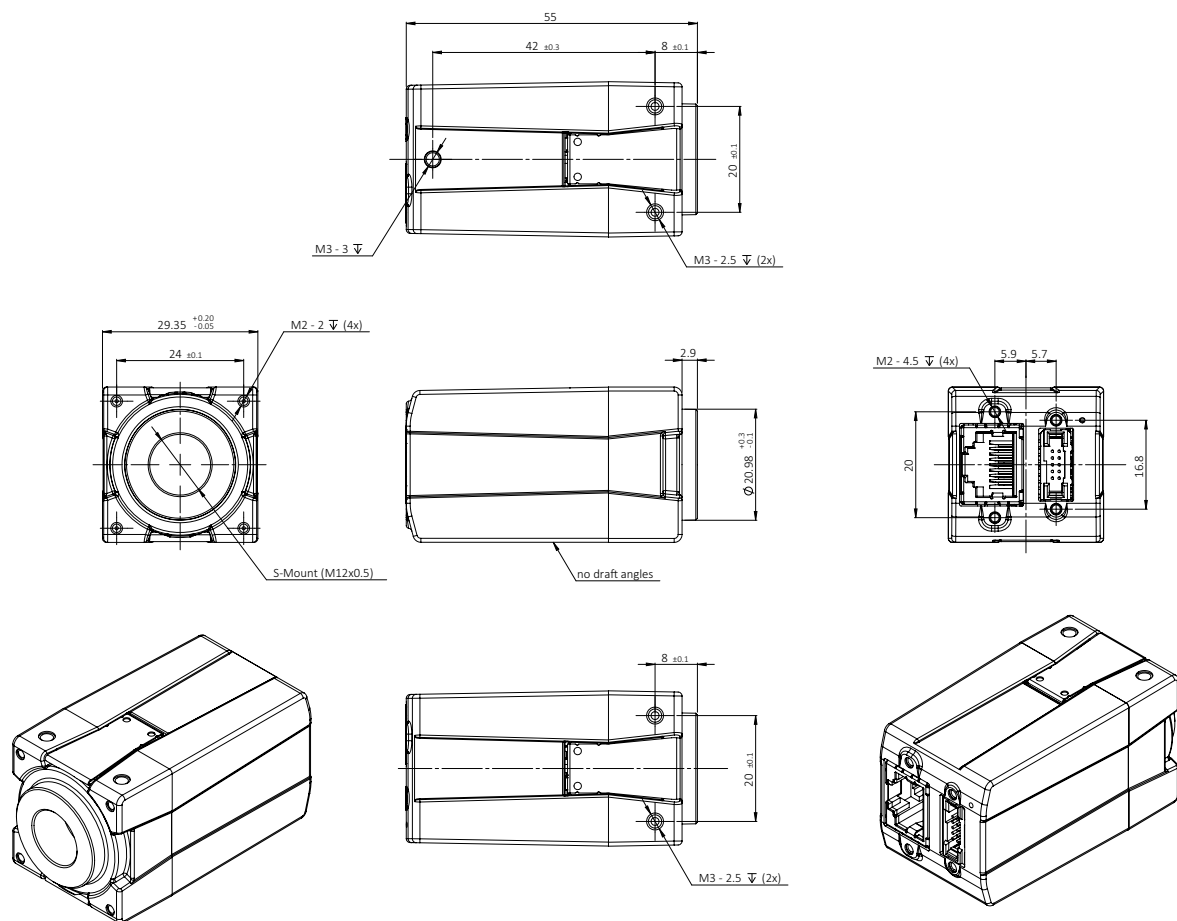
Figure 32: Dimensions for S-Mount models
