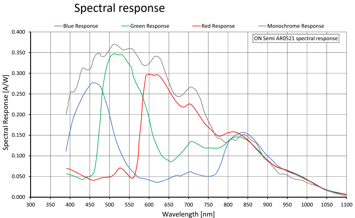
Figure 8: Alvim G5-500m/c (ON Semi AR0521) spectral response
