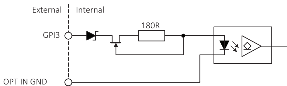
Figure 49: Input block diagram
