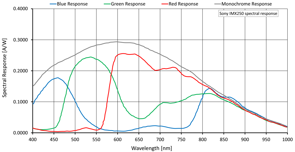
Figure 10: Alvium G5-508m/c (Sony IMX250) spectral response
