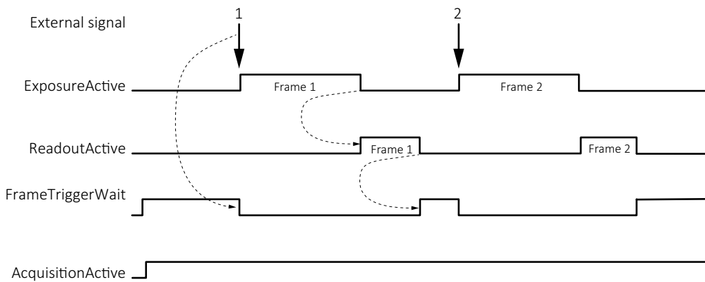
Figure 54: Schematic trigger signal flow
