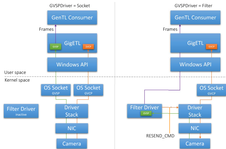
Figure 65: Stream handling with GVSPDriverSelector set to Socket or Filter
