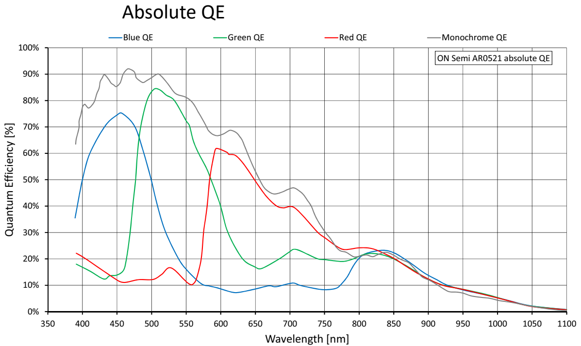
Figure 7: Alvim G5-500m/c (ON Semi AR0521) absolute QE
