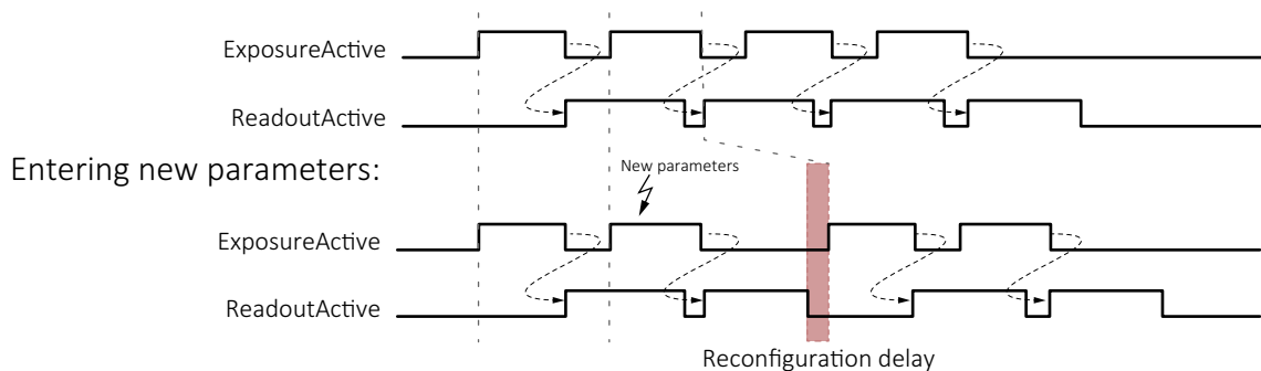
Figure 68: Delayed exposure due to parameter changes
