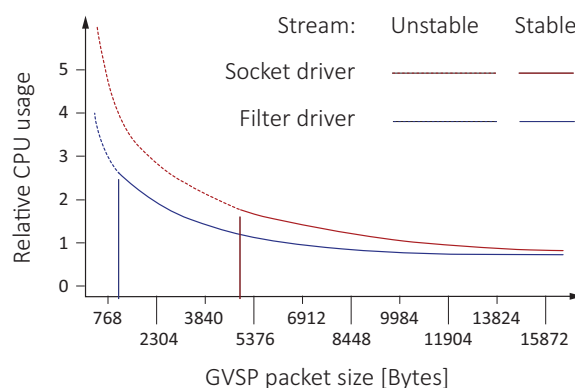
Figure 66: GVSPPacketSize versus CPU usage while the camera is streaming
