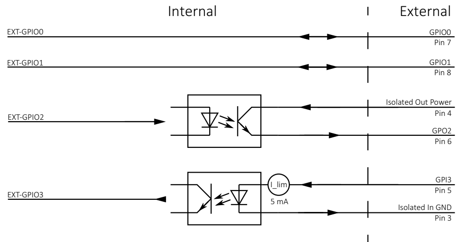
Figure 48: TFM I/O connector pin assignment
