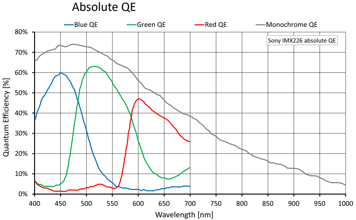
Figure 18: Alvium G5-1240m/c (Sony IMX226) absolute QE
