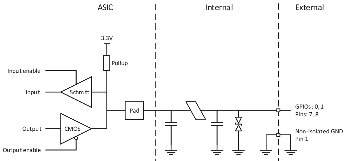
Figure 53: GPIOs block diagram
