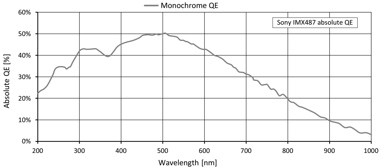
Figure 17: Alvium G5-812 UV (Sony IMX487) absolute QE
