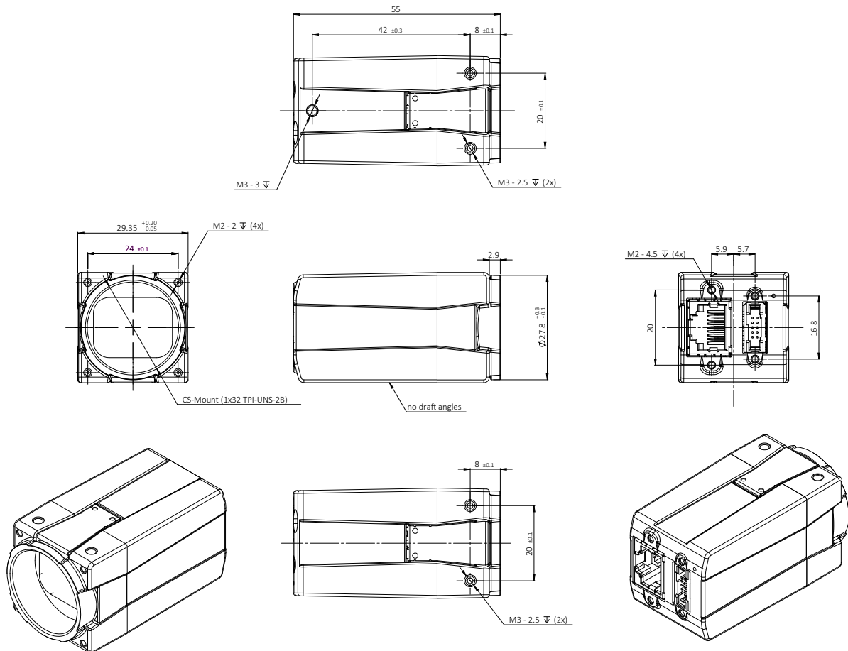
Figure 31: Dimensions for CS-Mount models
