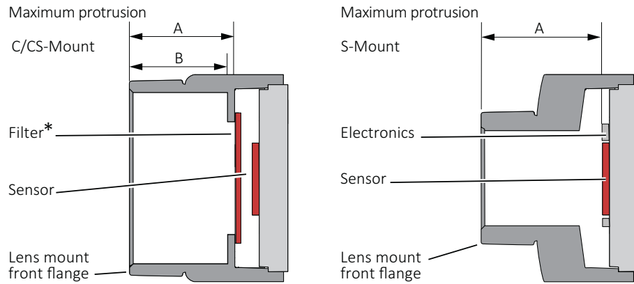
Figure 33: Maximum protrusion C-Mount, CS-Mount (left), and S-Mount (right)
