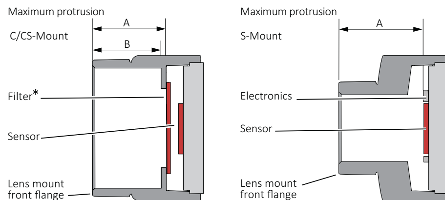
Figure 3: Maximum protrusion C-Mount/CS-Mount and S-Mount
