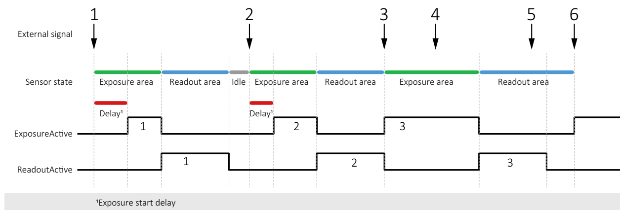
Figure 55: Triggering rolling shutter cameras
