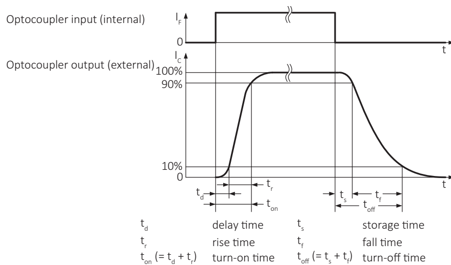
Figure 52: Output switching times
