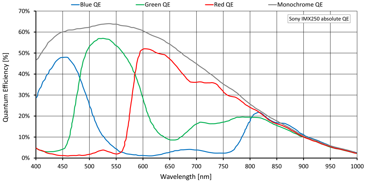
Figure 9: Alvium G5-508m/c (Sony IMX250) absolute QE
