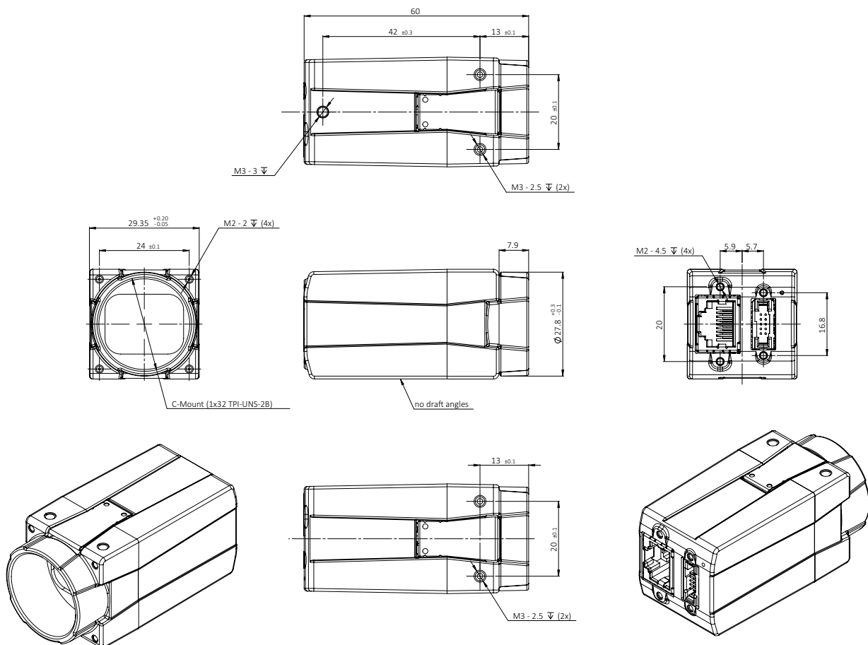
Figure 30: Dimensions for C-Mount models
