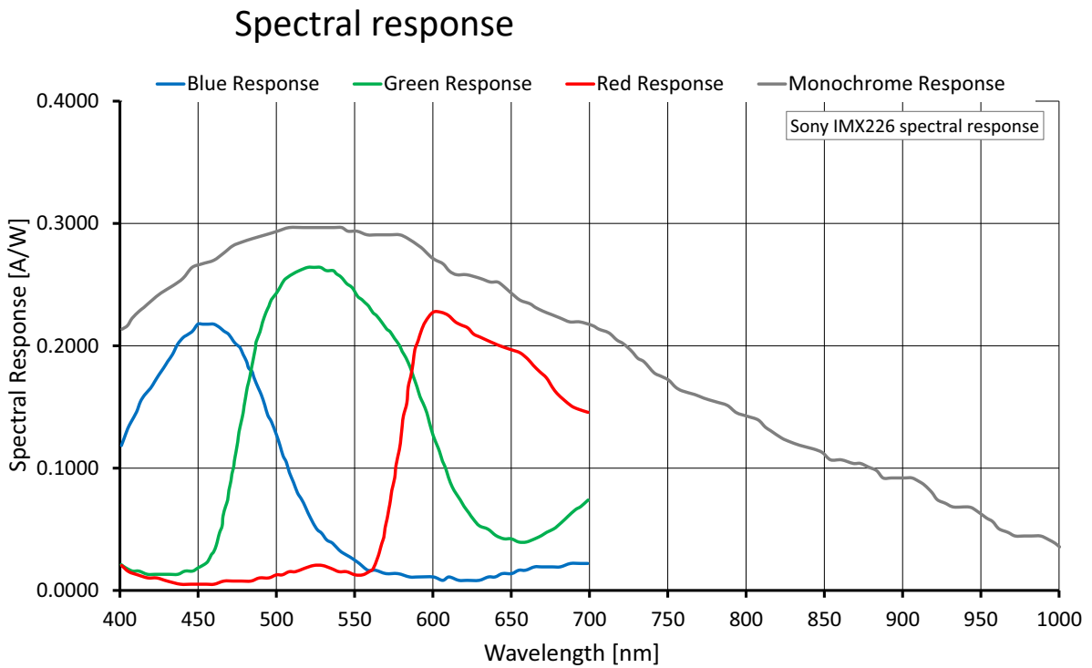
Figure 19: Alvium G5-1240m/c (Sony IMX226) spectral response
