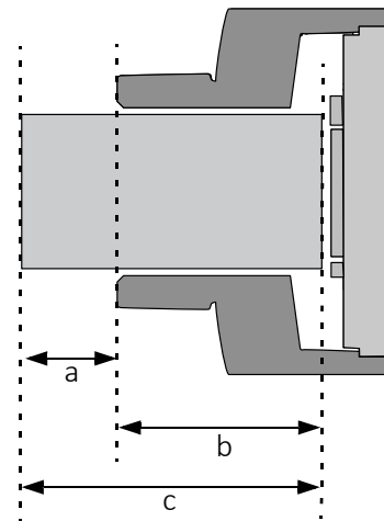
Figure 41: S-Mount lens and maximum protrusion
