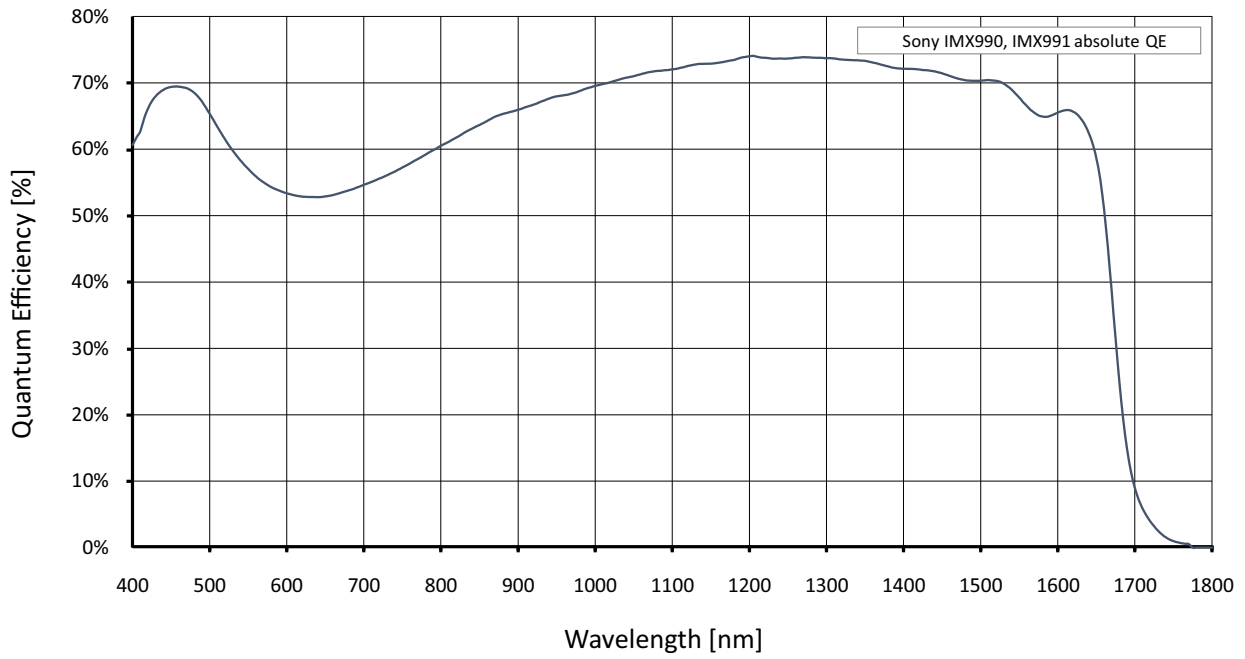
Figure 4: Alvium G5-130m SWIR (Sony IMX990) absolute QE
