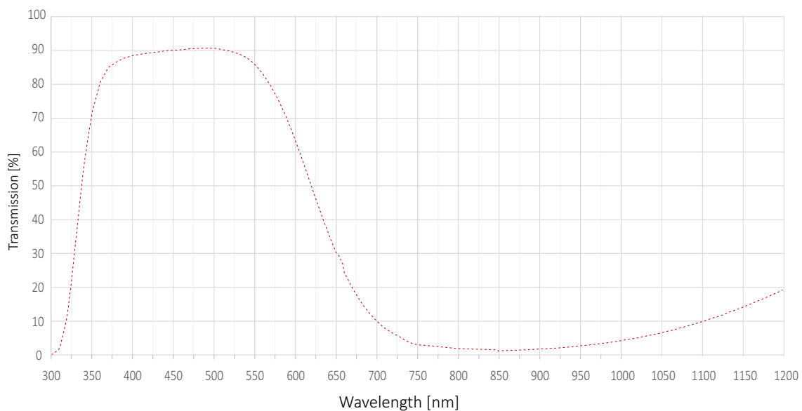
Figure 34: Spectral transmission for type Hoya C5000 IR cut filter (exemplary curve)
