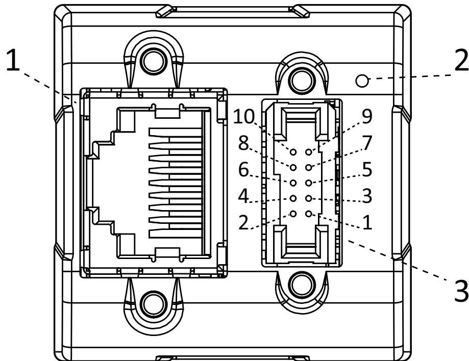
Figure 47: Back panel of camera
