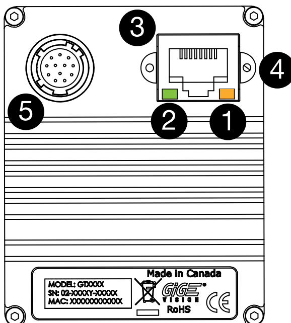
Figure 96: Port and LEDs (Large Format housing)
