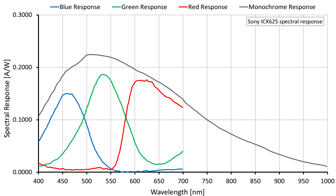
Figure 33: Prosilica GT2450 (Sony ICX625) spectral response
